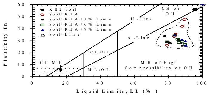
Figure 4. Plasticity chart of stabilized expansive soil
