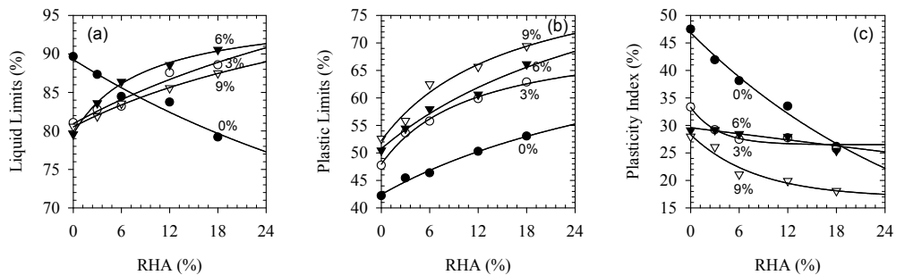
Figure 3. Effect of RHA addition on consistency limit of lime-stabilized expansive soil (Note: numbers in percents are referring to percentage of lime content).
